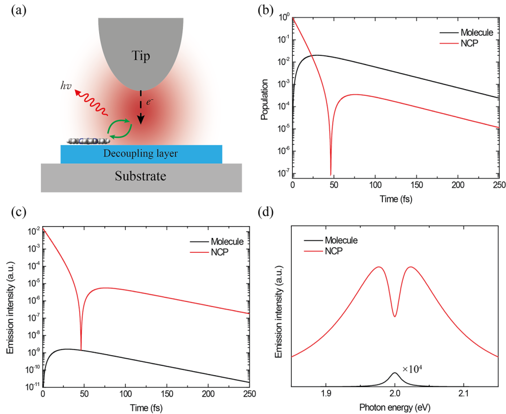
FIG. 2 (a) Schematic of STM induced NCP emission with the STM tip apex located in close proximity to the edge of a molecule. The molecule cannot be directly excited by tunneling electrons. Instead, the localized NCP in the junction can be excited by inelastic tunneling electrons. The time evolution of the populations (b) and emission intensities (c) of the NCP and the molecule after the NCP is initially excited. (d) Emission spectra for the molecule and the NCP when the NCP is selectively excited. The emission energy for both the molecule and the NCP is set to 2 eV.
