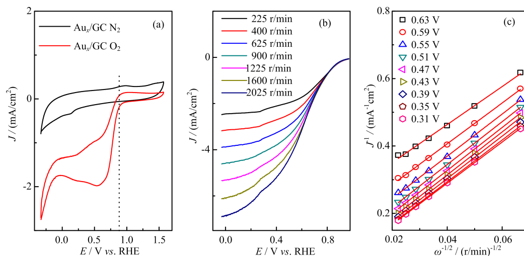
FIG. 4 (a) Cyclic voltammograms vs. RHE of the Au x /GC electrode in the N 2 - and O 2 -saturated 0.1 mol/L KOH aqueous solution at the potential scan rate of 0.1 V/s, (b) Linear-sweep voltammograms vs. RHE of the Au x /GC electrode at different rotation rates from 225 r/min to 2025 r/min in O 2 -saturated 0.1 mol/L KOH aqueous solution; and DC ramp 20 mV/s, (c) Koutecky-Levich plots at different potentials from 0.31 V to 0.63 V. Current density is normalized to the effective Au active surface areas. Symbols (FIG. 4(c)) are obtained from the experimental data of the according linear-sweep voltammograms (FIG. 4(b)), and lines are the linear regressions.
