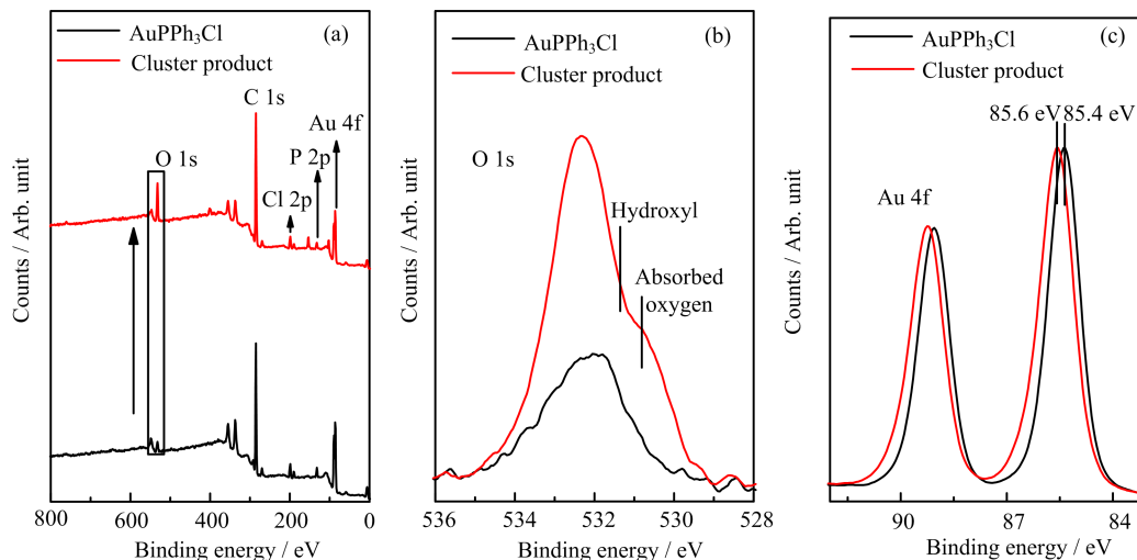
FIG. 3 (a) XPS survey, (b) high-resolution O 1s, (c) Au 4f spectra of the AuPPh 3 Cl and the cluster product.
