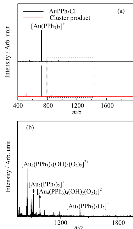
FIG. 1 (a) ESI-MS of the AuPPh 3 Cl and the Au_x cluster product over the range of m/z=400-2000 , (b) ESI-MS of the Au_x cluster product over the range of m/z=750-2000 .
