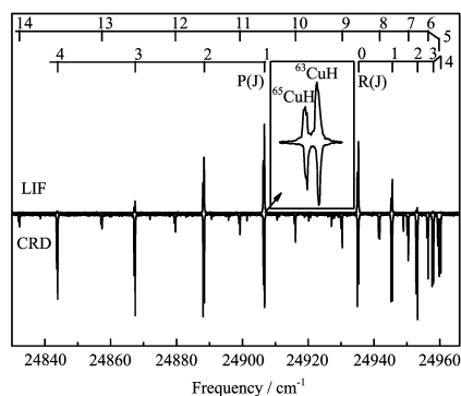
FIG. 1 LIF and CRD spectra of the A^1\Sigma^+-X^1\Sigma^+ (1, 0) band of CuH. The insert shows the zoomed-in of ^{63/65}\text{Cu} isotope resolved P(1) line in both spectra.
