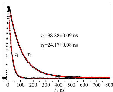
FIG. 2 Typical fluorescence signals of P(1) and P(2) transitions in the A^1\Sigma^+-X^1\Sigma^+ (0, 0) band of CuH. The red traces represent the mono-exponential fits, from which upper state lifetimes ( \tau_0 and \tau_1 ) are determined. Errors given in figure are one standard deviation of the fits, which is much smaller than the pulse duration of the dye laser used in the present experiment.
