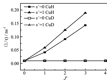
FIG. 3 Plots of 1/\tau versus rotational quantum number J' for both CuH and CuD.
