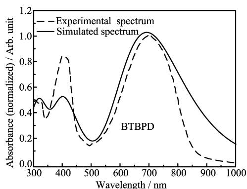
FIG. 4 Simulated and experimental absorption spectra for BTBPD in solid state.
