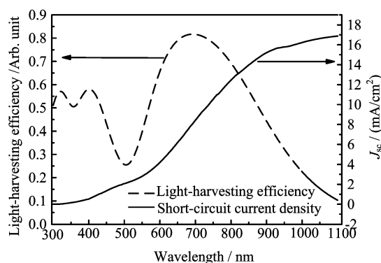
FIG. 5 Predicted J_{sc} and \eta_{\lambda} for BTBPD-PC 61 BM cell.
