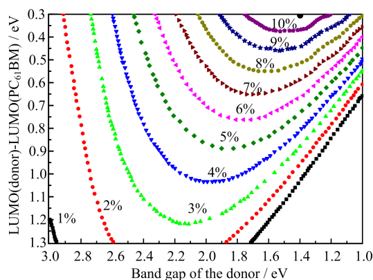
FIG. 3 Predicted PCE for BTBPD-PC 61 BM cell with the Scharber diagram.
