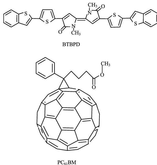
FIG. 1 Molecular structures of BTBPD and PC 61 BM.
