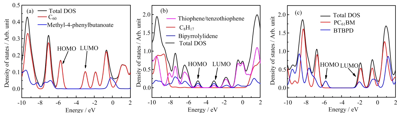
FIG. 2 Total density of states and partial density of states of (a) PC 61 BM, (b) BTBPD, and (c) PC 61 BM-BTBPD complex.
