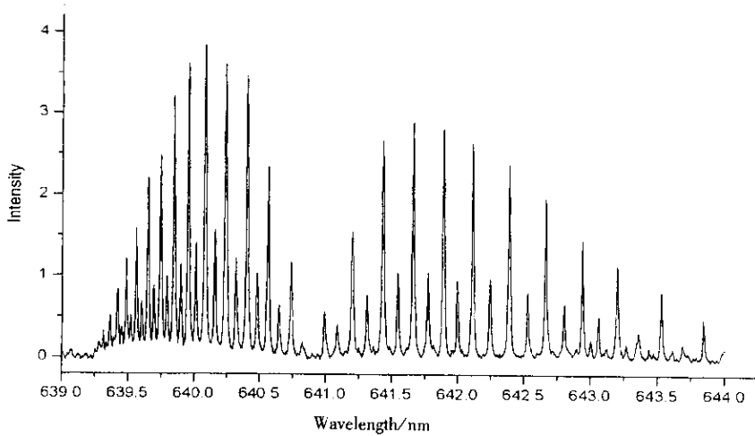
图 3 C 2 H 2 X 1 Σ g + (2030 0 0 0 )←(0000 0 0 0 )跃迁的脉冲光声光谱
