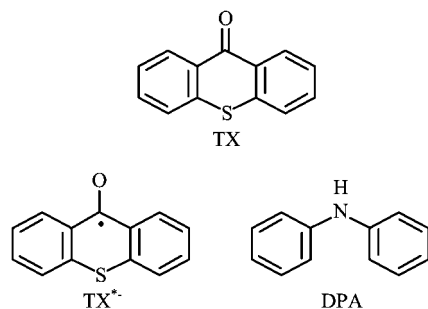
Scheme 1 Molecular structures of TX, TX \cdot^- , and DPA.
