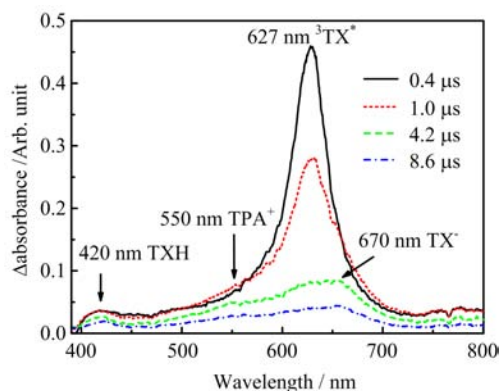
FIG. 6 Transient absorption spectra of TX and TPA in pure \text{CH}_3\text{CN} at different delay time after photolysis.
