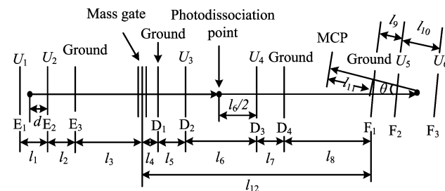
FIG. 2 Simple diagram of the basic dimensions and electric voltages. l_1=l_2=3 cm, d=2 cm, l_3=66.1 cm, l_4=0.1 cm, l_5=0.4 cm, l_6=1.8 cm, l_7=0.4 cm, l_8=67.5 cm, l_9=9.7 cm, l_{10}=13 cm, l_{11}=43.5 cm, and l_{12}=70.2 cm.
